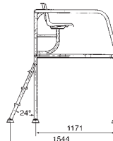
Bokorys
